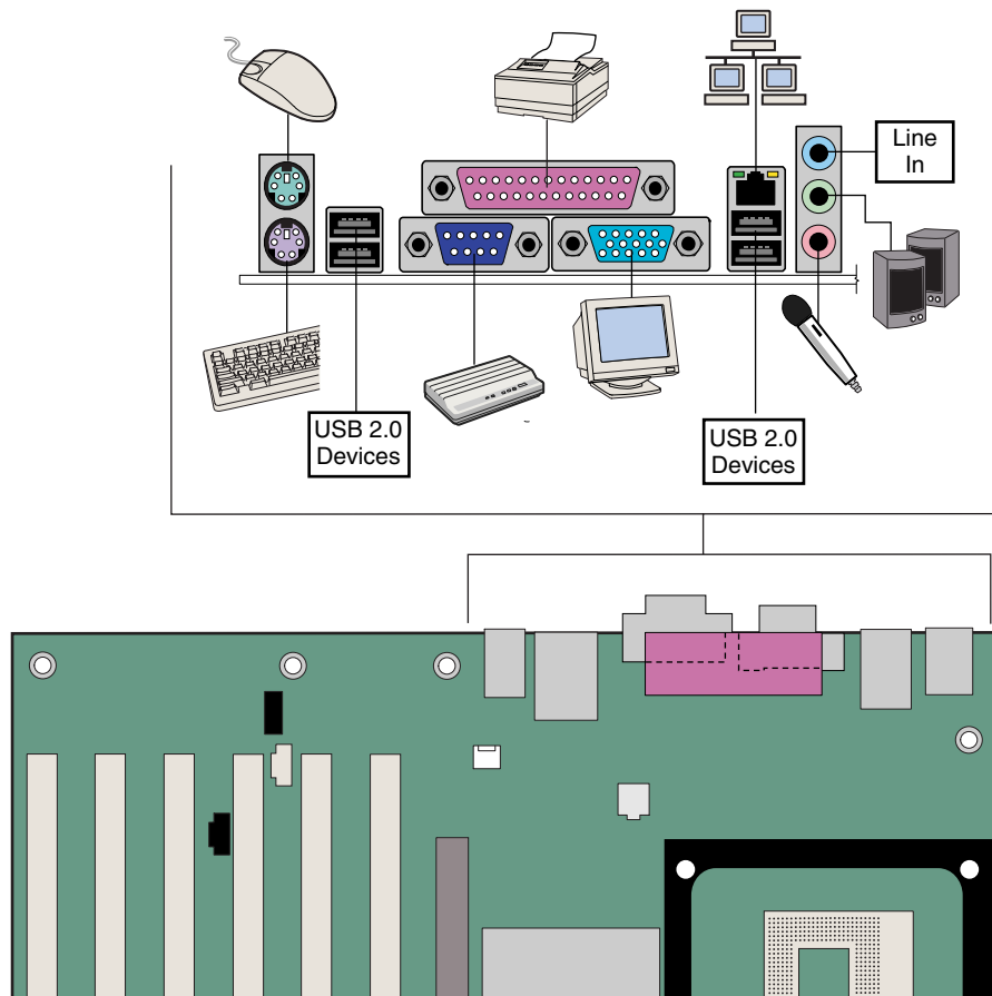
Figure 18. Back Panel Connectors
